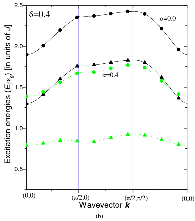
Figure 6. The elementary excitation dispersion relations of the ferrimagnetic system (1, \frac{1}{2}) on a square lattice. The spectra are shown for different \alpha and for (a) \delta = 0.0 and (b) \delta = 0.4 . Curves with circles represent optical modes while curves with triangles represent acoustic ones.
