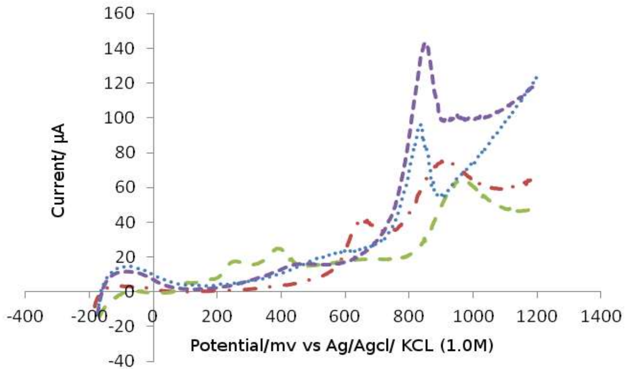
Figure 1. Differential pulse voltammograms platinum electrodes modified by Bismuth, platinum electrode. Scan rate: 10 mV/s.
