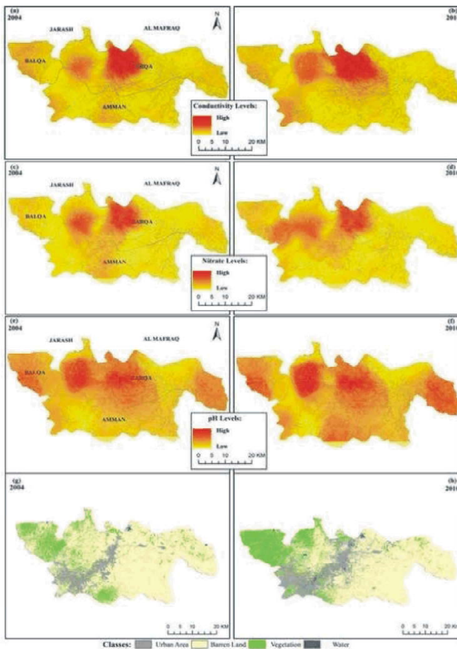
Fig. 2: Changes in conductivity, nitrate and pH hotspot levels and the land use land and cover changes between 2004 and 2010
